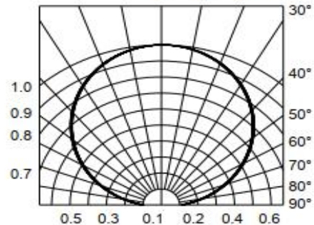
Fig.6-Radiation Diagram Ta=25°C
